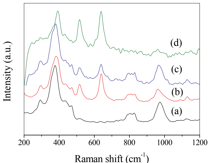
Fig. 7. Raman spectra of TS-1/CNF composites after removing CNFs.
