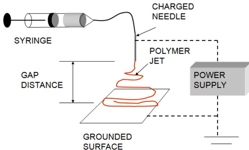
Fig. 1. Electrospinning setup.
