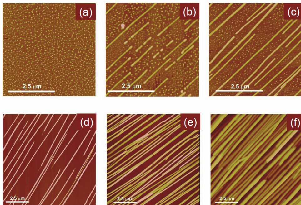
Fig. 1. AFM topography images of p -6P nanofiber films grown by hot-wall epitaxy on (001)-oriented muscovite mica with (a) 10 s, (b) 25 s, (c) 90 s, (d) 5 min., (e) 40 min., and (f) 120 min. deposition time. The growth temperature is 130 °C. The height scale is 0–50 nm in (a)–(c), 0–100 nm in (d), 0–220 nm in (e), and 0–700 nm in (f).
