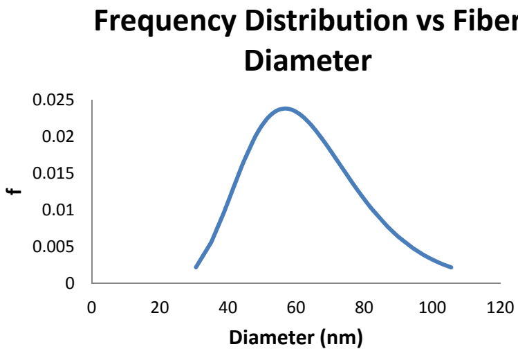
Fig. 12. Length weighted log-normal fiber diameter frequency distribution of of \text{Rh}_2\text{O}_3/\text{Al}_2\text{O}_3 nanofibers.
