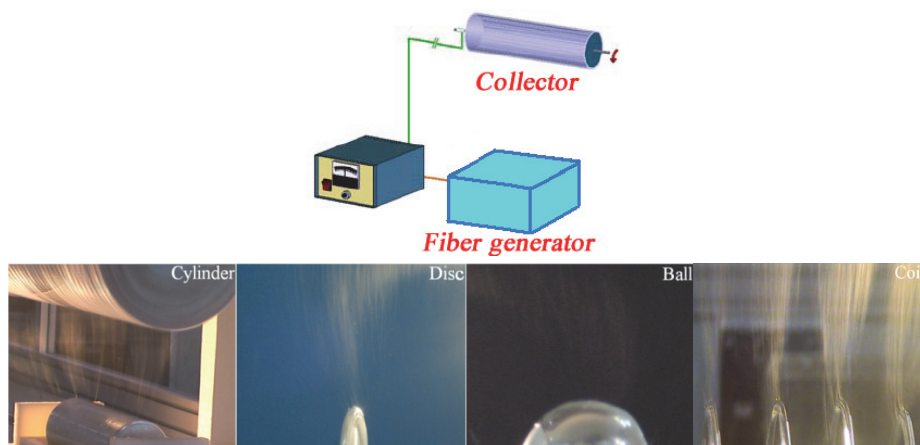
Fig. 11. Schematic illustrations of needleless electrospinning setup, and cylinder, disc, ball, and spiral coil electrospinning processes (Niu et al. , 2009; Lin et al. , 2010).
