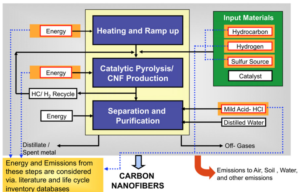
Fig. 2. LCA of Carbon Nanofibers: System Boundary.
