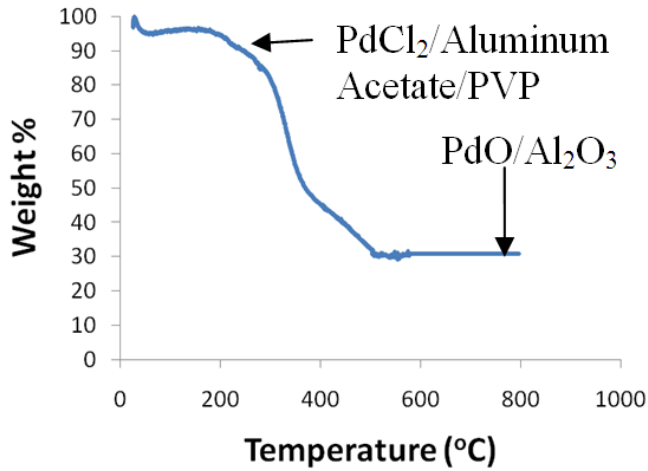
Fig. 3. TGA of PdCl 2 /Aluminum Acetate/PVP nanofibers.
