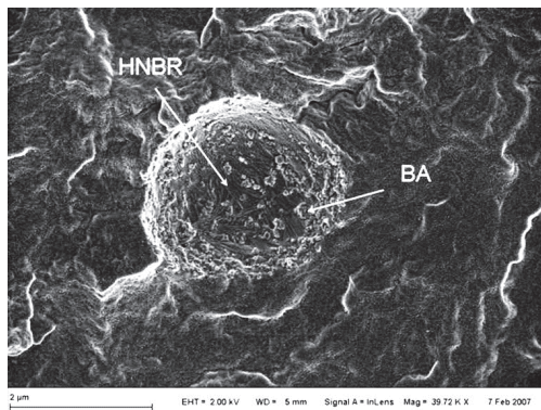
Fig. 9. SEM image of PA-6/HNBRBA ternary composite (Siengchin & Karger-Kocsis, 2009).
