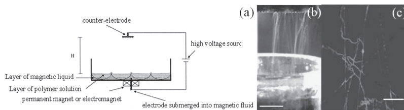
Fig. 8. (a) A two-layer-fluid electrospinning setup, (b) multiple jets ejected toward the counter-electrode, (c) an image of as-spun fibers (scale bar is 50 mm) (Yarin & Zussman, 2004).
