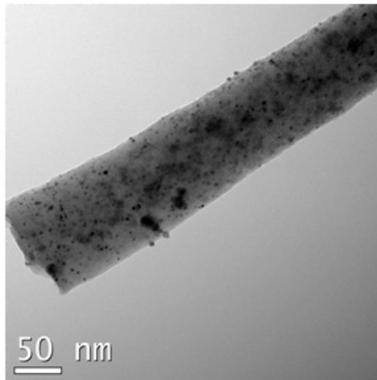
Fig. 6. Transmission electron micrographs of PdO/Al 2 O 3 nanofibers.
