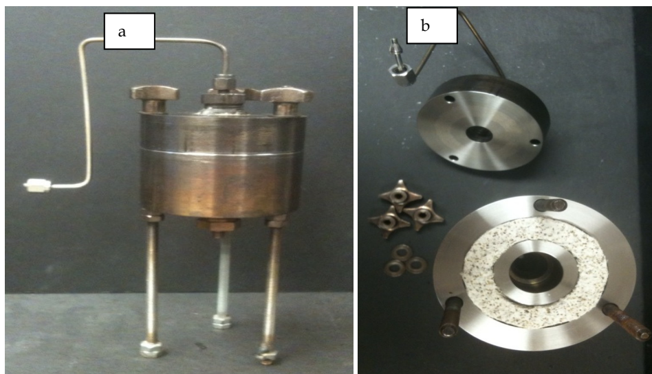
Fig. 16. (a) Reactor (b) Internal view of the reactor and screws.
