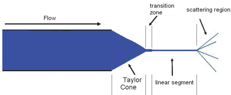
Fig. 12. Representation of fluid deformation in electrospinning process.
