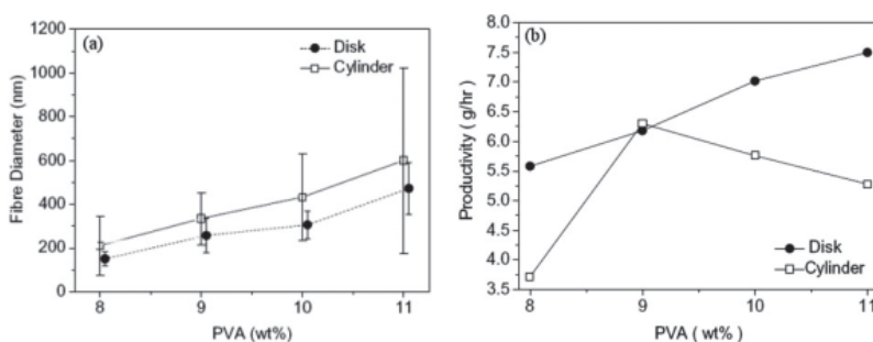
Fig. 15. Influence of PVA concentration on (a) fiber diameter, and (b) fiber productivity (collecting distance = 13 cm, applied voltage = 57 kV, cylinder diameter = 80 mm, cylinder rim radius = 2 mm, disc diameter = 80 mm, disc thickness = 2 mm) (Niu et al. , 2009).
