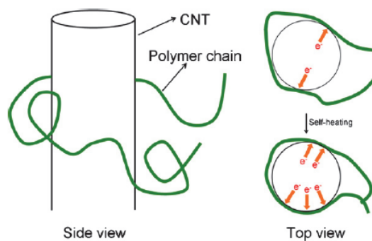
Fig. 15. Schematic representation illustrating the self-heating phenomena between a CNT and a polymer chain inside a conducting composite electrospun nanofiber [121].
