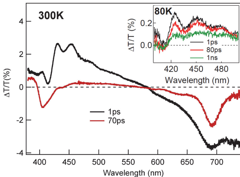
Fig. 8. Differential transmission spectra of p -6P epitaxial nanofibers excited by ultrafast pulses centered at 360 nm, for different lattice temperatures and pump-probe time delays. Pump pulsed fluence: 90 \mu\text{J}/\text{cm}^2 (main panel); 10 \mu\text{J}/\text{cm}^2 (inset).
