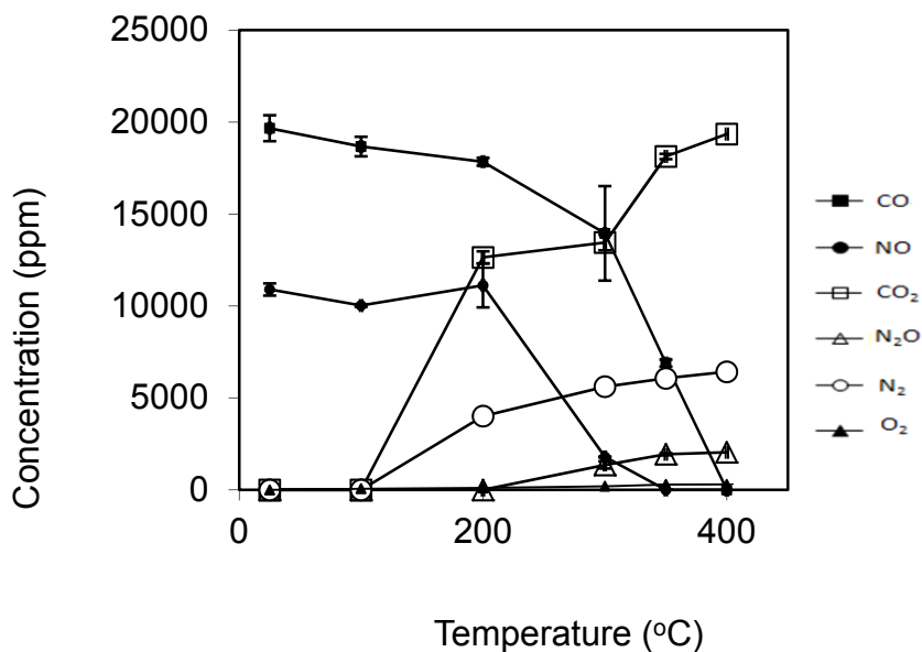
Fig. 18. Concentration vs. temperature for the reaction over 0.05g of Pd/Al 2 O 3 .
