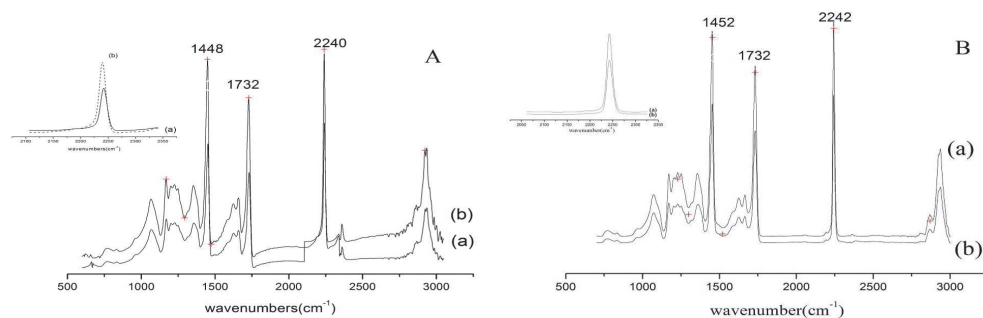
Fig. 13. Polarized FTIR spectra of PAN nanofiber: (A) before and (B) after hot-stretching, absorbent spectra at the perpendicular (a) and parallel (b) directions respectively.
