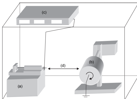
Fig. 11. A typical setup used to produce nanofibers by electrospinning. (a) Injection pump with hypodermic syringe; (b) grounded collector; (c) high voltage supply; and (d) working distance.
