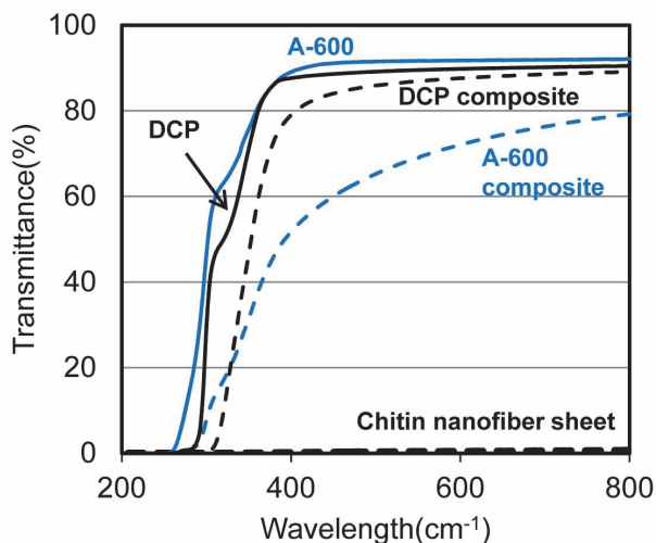
Fig. 16. Regular light transmittance spectra of neat acrylic resins (solid lines) and their nanocomposites (dashed lines).
