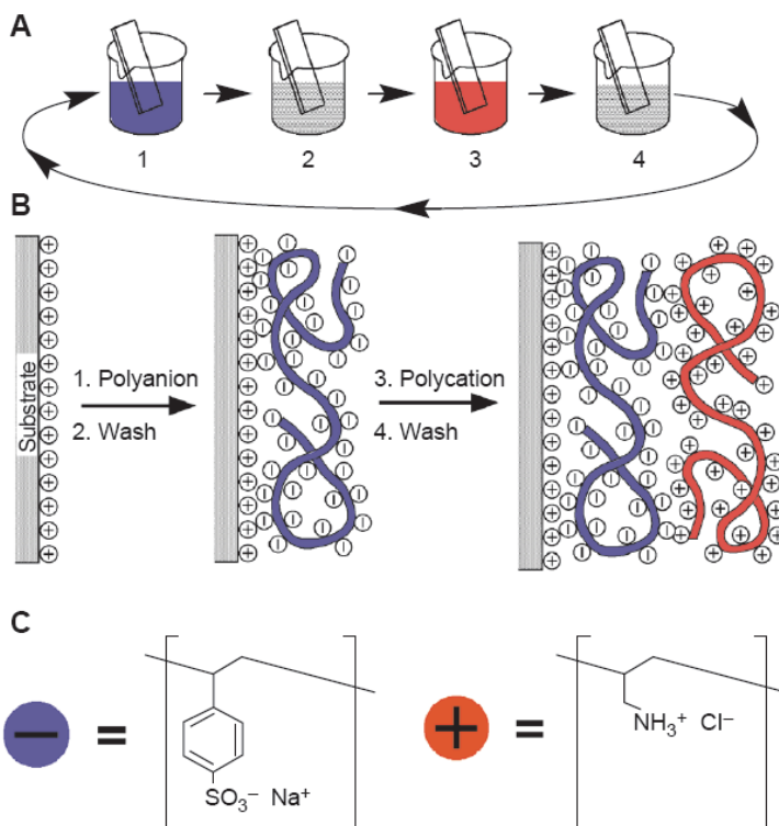
Fig. 8. Schematic of the film deposition by the LBL process according to Decher [41].
