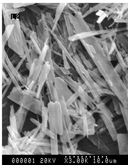
Fig. 6. \text{MoO}_3 morphology synthesized at 0.5 moles ratio of CTAB with AHM under 180°C for 40h.
