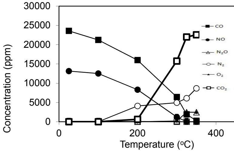
Fig. 19. Concentration vs. temperature for the reaction over 0.05g of Pt/Al 2 O 3 .
