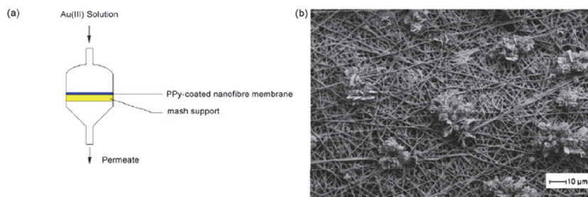
Fig. 4. (a) Apparatus for mat-based Au recovering, (b) SEM image of the PPy-coated nanofibers with aqueous [\text{Au}(\text{III})\text{Cl}_4]^- solution permeated (Wang et al., 2007).
