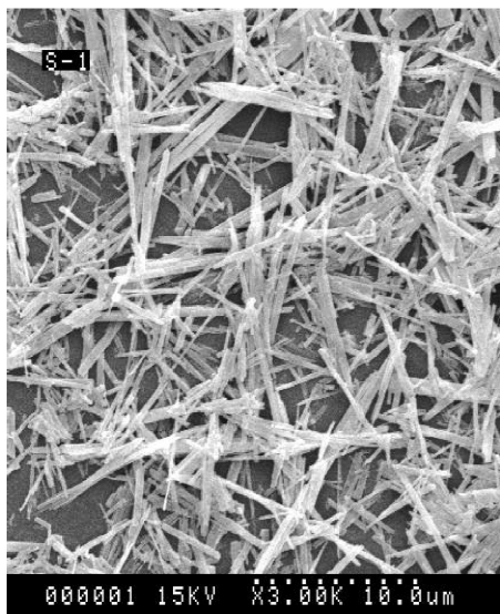
Fig. 9. MoO 3 morphology of precursor of 25% AHM at acidity coefficient 15(180°C for 40h).
