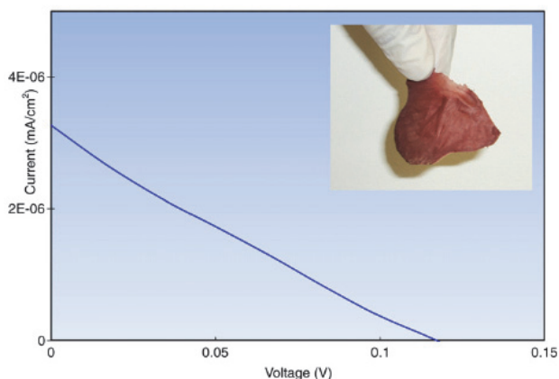
Fig. 18. J_{sc} -V graph of the P3HT/PCBM solar cloth measured under 1 Sun conditions. Inset shows a picture of the solar cloth fabricated using electrospinning [105].
