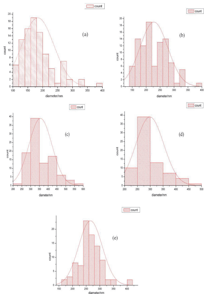
Fig. 9. The diameter distribution of PAN and PAN/SWNTs nanofibers with different SWNTs concentration (a)0wt% (b)0.25wt% (c)0.5wt% (d)0.75wt% (e)1wt%.
