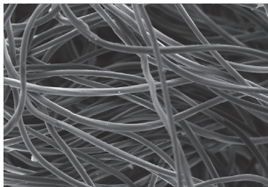
Fig. 1. Scanning electron micrograph (SEM) image of nanofibers.
