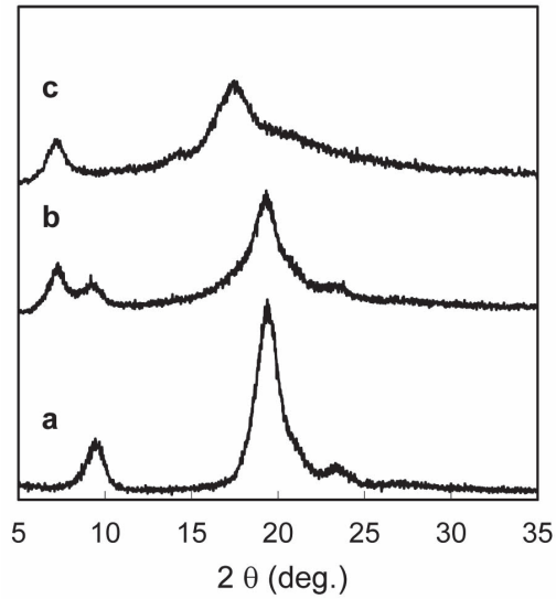
Fig. 21. X-ray diffraction profiles of acetylated chitin nanofibers of (a) DS 0.99, (b) DS 1.81, and (c) DS 2.96.
