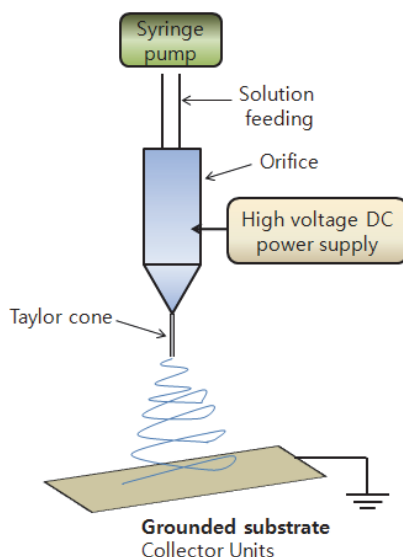
Fig. 2. Schematic image of the electrospinning method.
