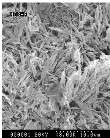
Fig. 8. \text{MoO}_3 morphology synthesized at 1.0 moles ratio of CTAB with AHM under 180^\circ\text{C} for 40h.
