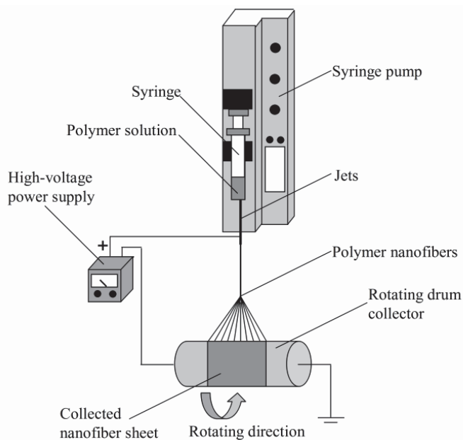
Fig. 1. Schematic diagram of the electrospinning technique.
