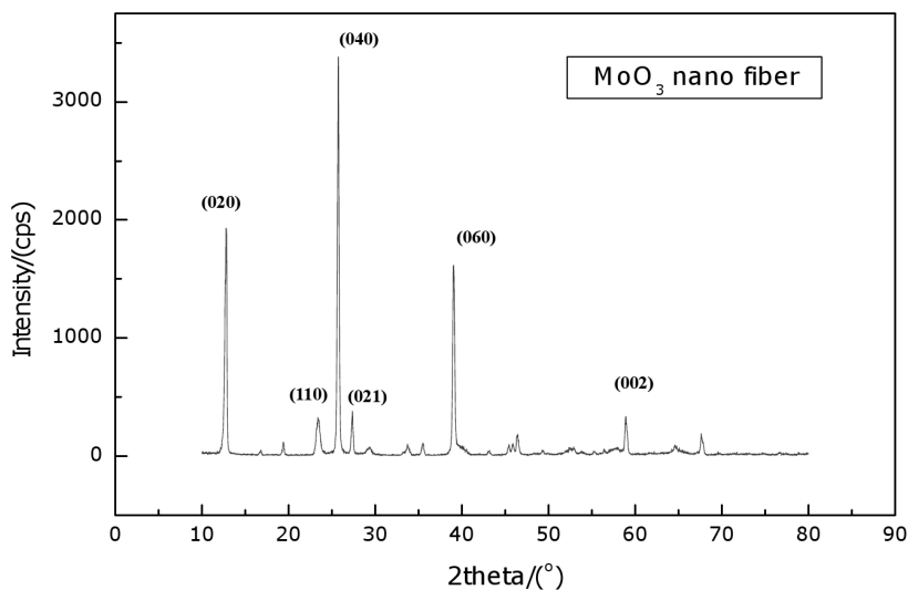
Fig. 16. The XRD patterns of MoO 3 nano fibers.
