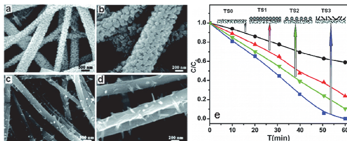
Fig. 5. SEM images of different \text{SnO}_2 morphologies on \text{TiO}_2 nanofibers (a-d) and the \text{SnO}_2 morphology dependent photocatalytic degradation behavior of Rhodamine B (e) (Wang et al., 2009a).
