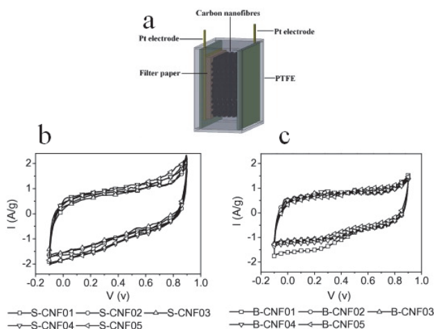
Fig. 7. (a) Illustration of electrochemical cell and the cyclic voltammety curves of side-by-side (b) and blend (c) carbon nanofibers (Niu et al., 2011).
