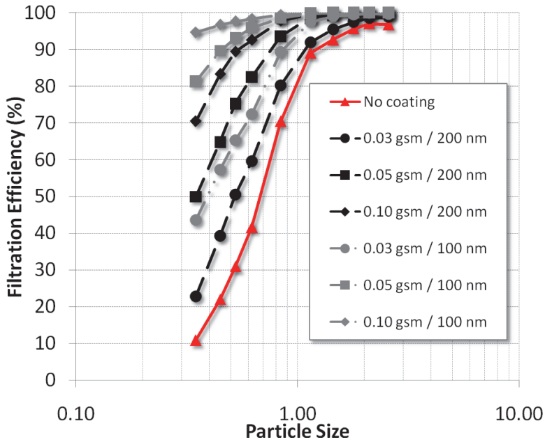
Fig. 11. Filtration efficiency of nanofiber media samples.
