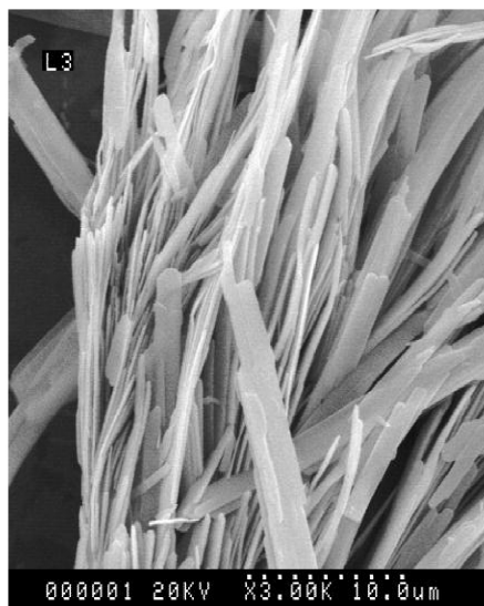
Fig. 7. \text{MoO}_3 morphology synthesized at 0.7 moles ratio of CTAB with AHM under 180^\circ\text{C} for 40h.
