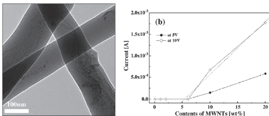
Fig. 16. TEM image of the MWNTs/nylon composite nanofibers with 10 wt.% and its I-V characteristics plot [122].
