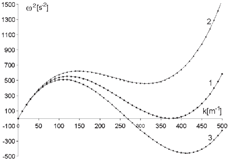
Fig. 5. Relationship between the square of the angular frequency and the wave number for distilled water, electric field is the parameter 1: E = E_c = 2.461\ 945\ 094 \times 10^6 V/m, 2: E = 2.4 \times 10^6 V/m, and 3: E = 2.5 \times 10^6 V/m (Lukas et al., 2008).
