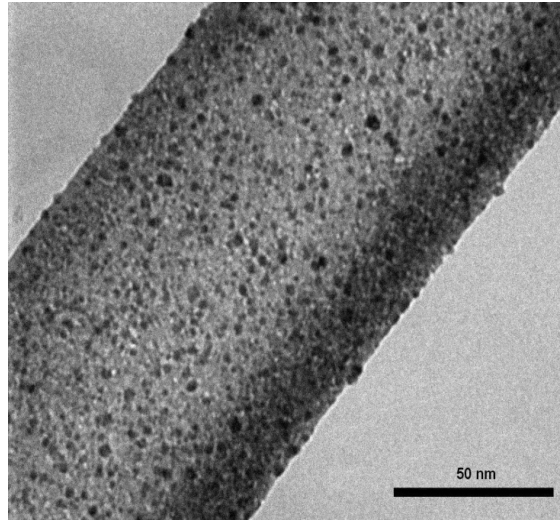
Fig. 11. Transmission electron micrograph of \text{Rh}_2\text{O}_3/\text{Al}_2\text{O}_3 nanofibers.
