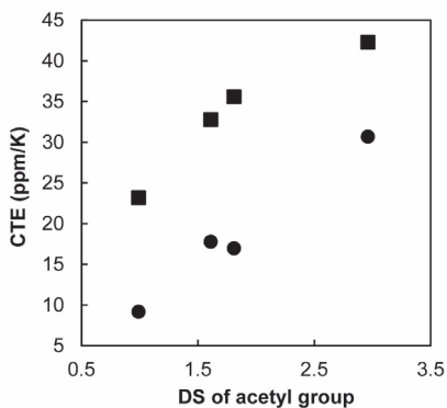
Fig. 26. Coefficient of thermal expansion of a series of acetylated chitin nanofibers (circles) and their nanocomposites (squares).
