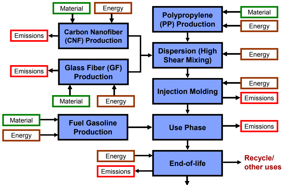
Fig. 5. Typical Life Cycle of a Polymer Nanocomposite.
