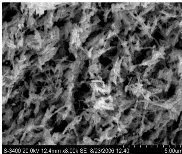
Fig. 22. SEM image of needle-like metal Mo powder.
