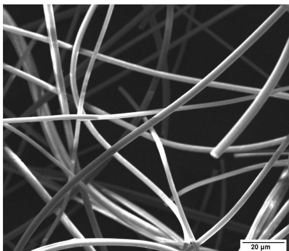
Fig. 13. Scanning electron micrographs of \text{Al}_2\text{O}_3 microfibers.
