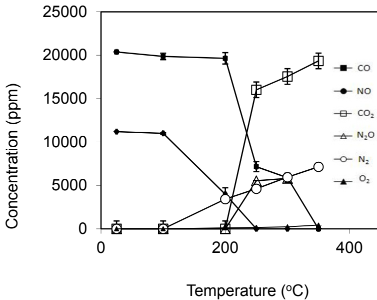
Fig. 20. Concentration vs. temperature for the reaction over 0.05g of Rh/Al 2 O 3 .
