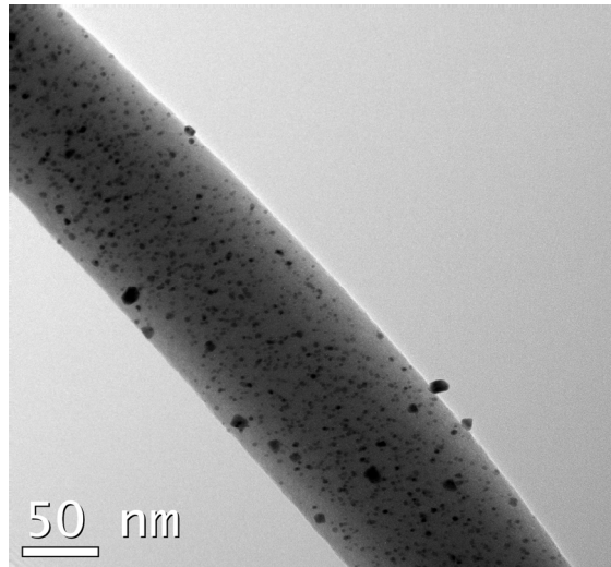
Fig. 8. Transmission electron micrographs of PtO/Al 2 O 3 nanofibers.
