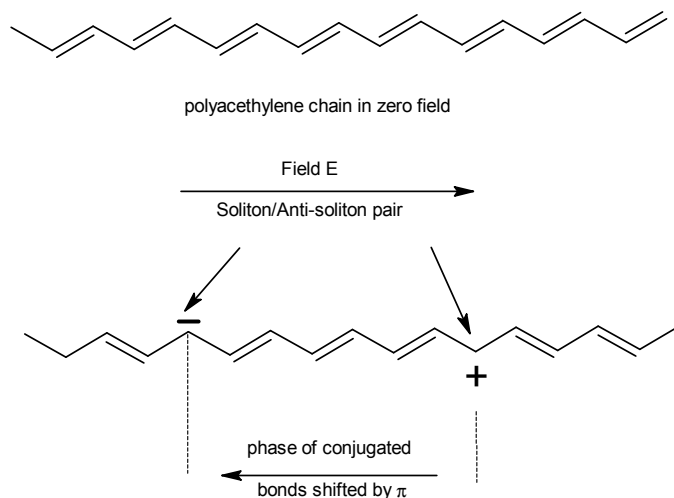
Fig. 4. Schematic representation of soliton - anti-soliton separation and electrical conduction in Polyacetylene chain. (source: http://electrons.wikidot.com ).
