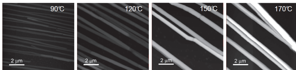
Fig. 2. Topographic images of the surface morphology of p -6P nanofiber films grown by hot-wall epitaxy on (001)-oriented muscovite mica at different substrate temperatures and with 60 min. deposition time. The height scale is 0–500 nm.
