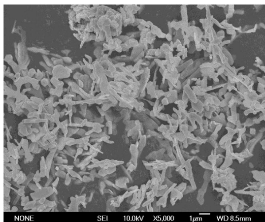
Fig. 20. The SEM image of nanofibers molybdenum trioxide reduction at 530°C for 1h.
